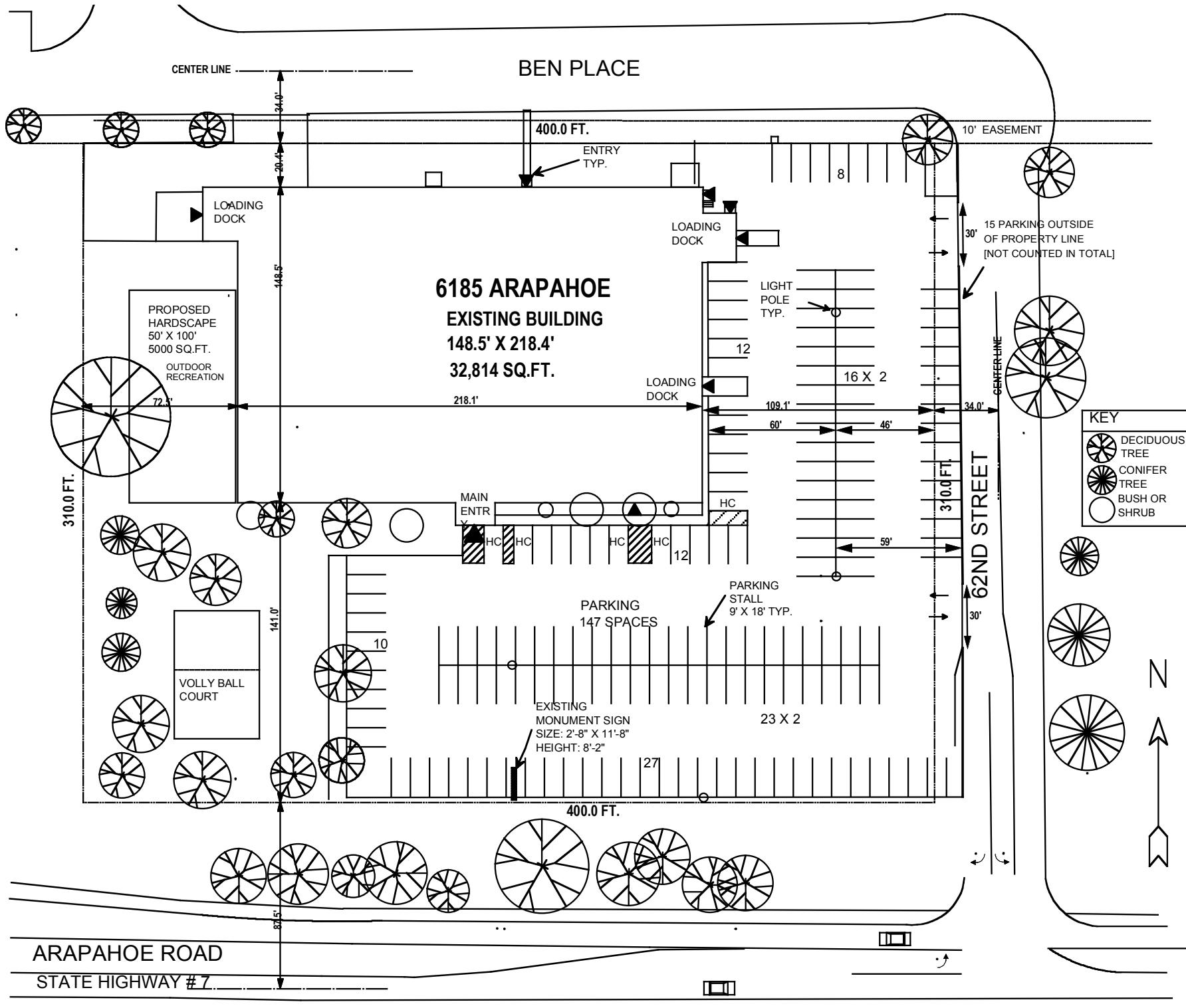
SITE PLAN SCALE: 1" = 60 FT.
